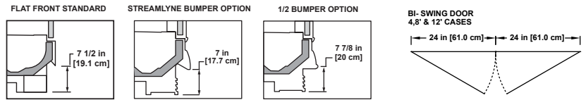
Door and Front Options Consult Hillphoenix Engineering Reference Manual for more available options.
