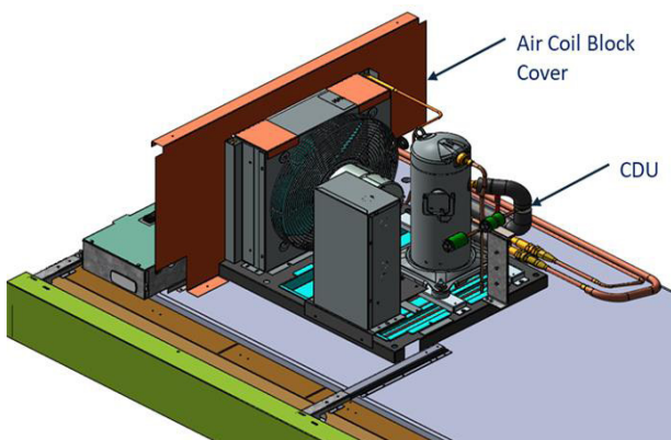
Fig. 22 Installed CDU with air block
