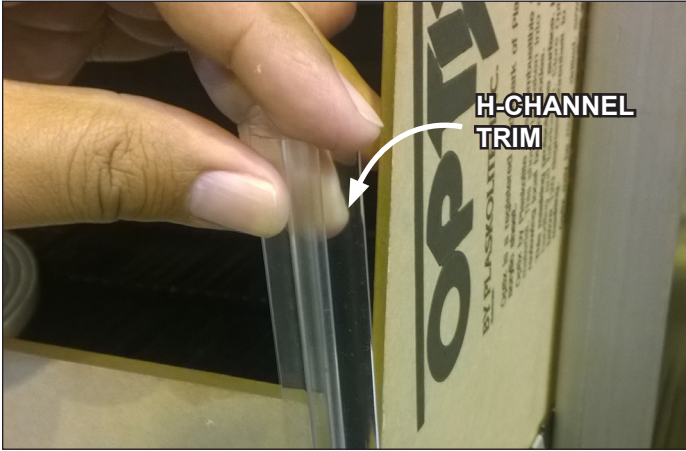
Fig. 10 H-channel trim joins front sill glass pieces
