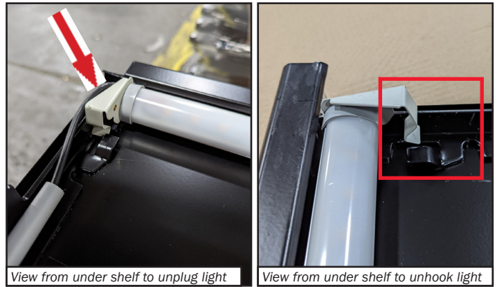
View from under shelf to unplug light View from under shelf to unhook light Fig. 25 Removing shelf lights
