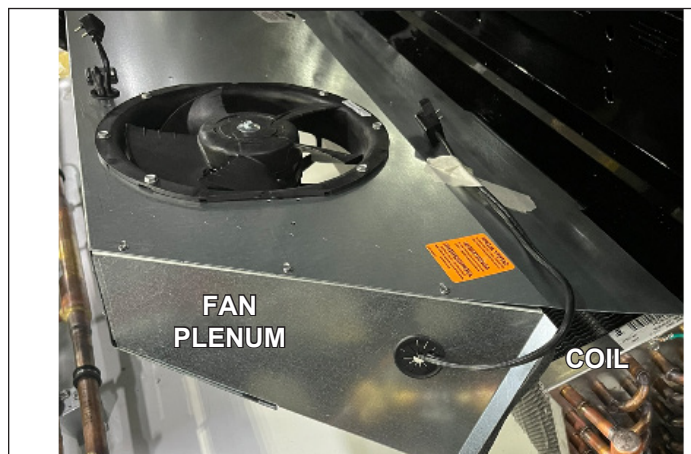
Fig. 30 Single-piece fan plenum and coil cover
