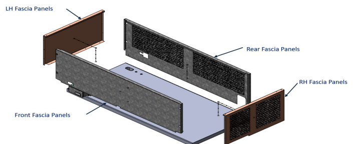
Fig. 20 Canopy level paneling
