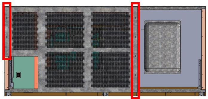
Fig. 19 6' case canopy view
