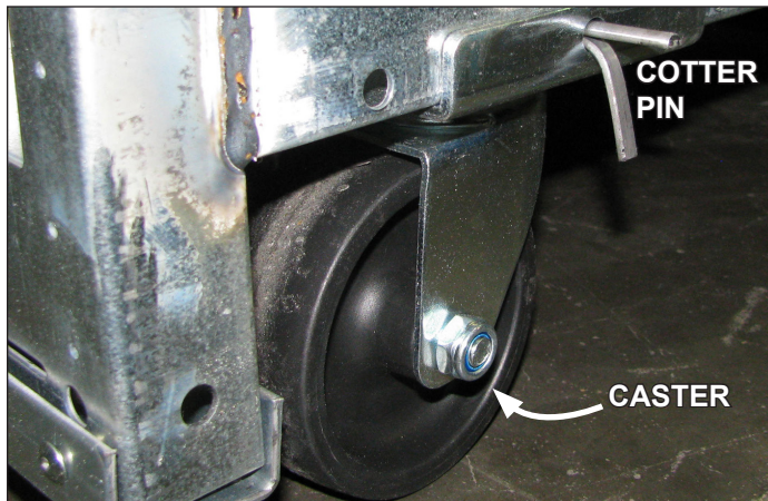
Fig. 1 Flatten and remove the cotter pins that are holding the casters in place, then lift the case with a "J" bar and slide the caster assemblies out. The dismantled casters can now be discarded.
