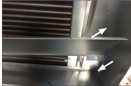
Fig. 2 Attach the bottom of the fascia baffle to the coil shroud.
