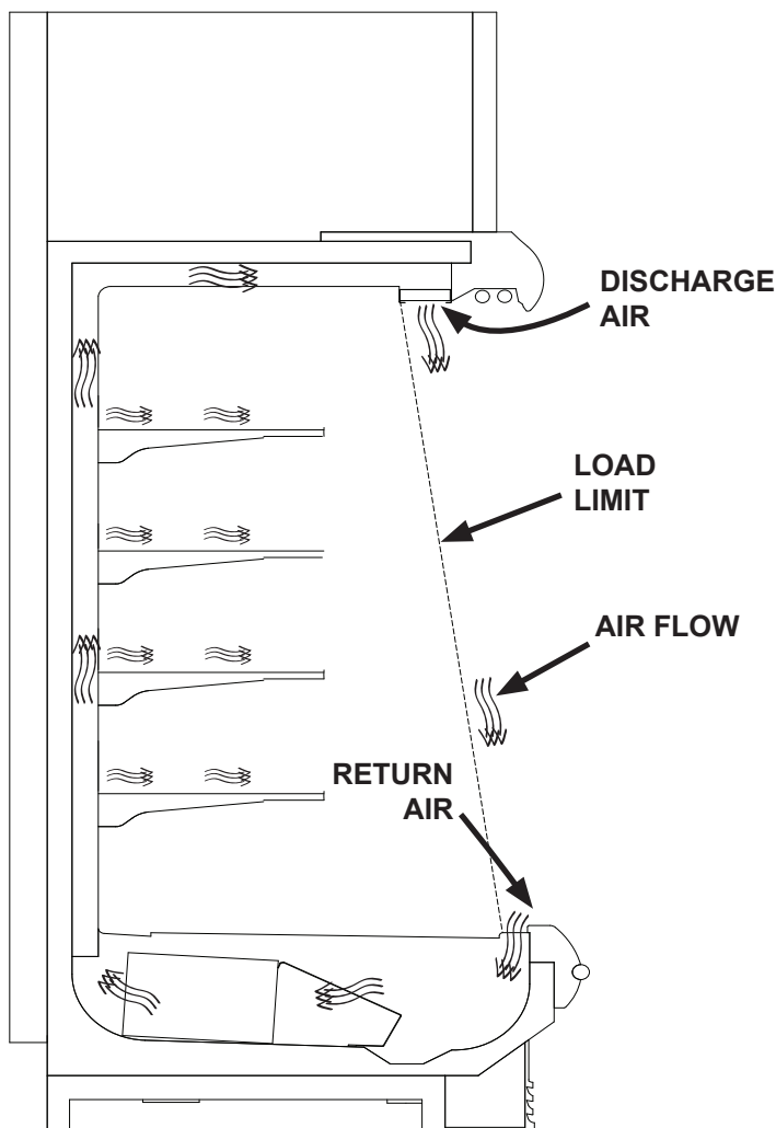
Fig. 28 Airflow
