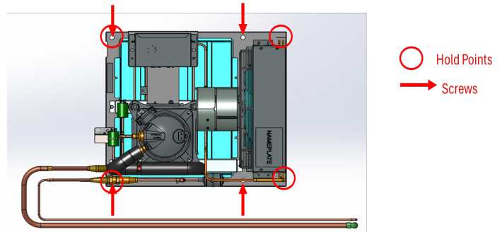
Fig. 23 CDU mounting locations and hold points
