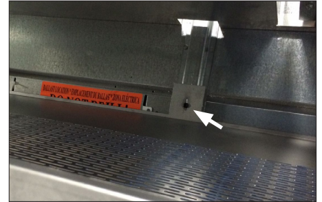
Fig. 3 Attach the bottom of the front fascia to the cornice assembly.
