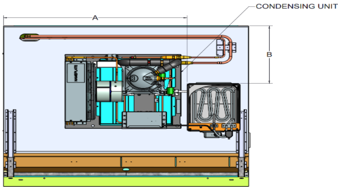
Fig. 21 Electric drain pan location
