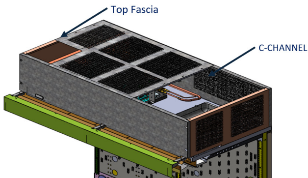
Fig. 17 Top fascia panel
