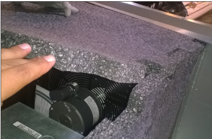
Fig. 3 Top panel installs under metal edge, fitting into pre-cut slots.
