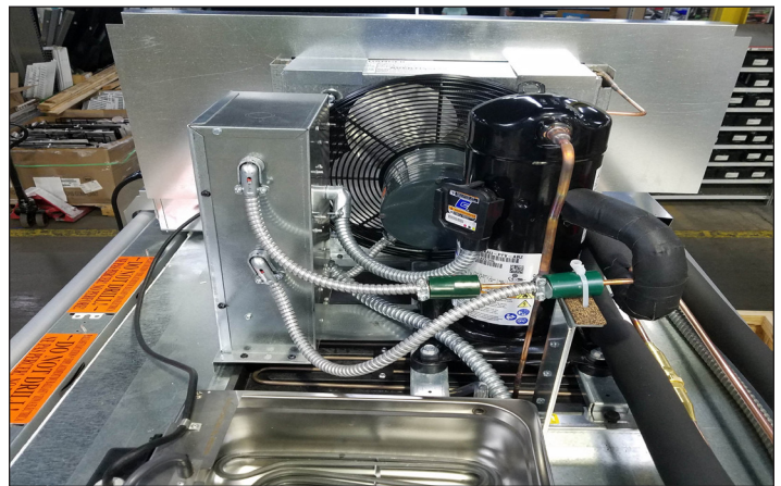
Fig. 12 Condensing unit on top of case
