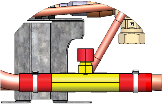
Fig. 31 Schrader port locations
