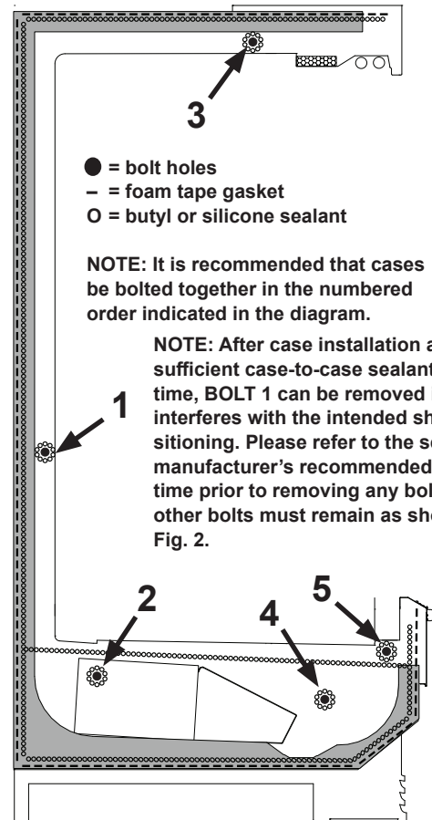
Fig. 2 Bolt holes, foam tape gasket, and sealant
