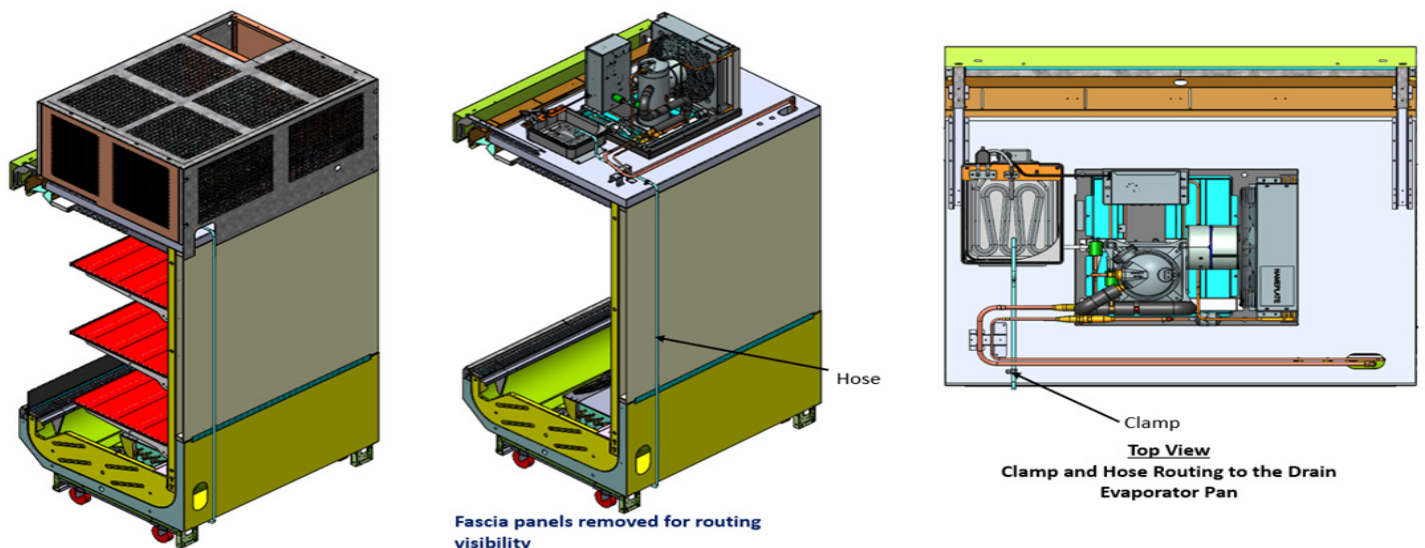
Fig. 4 Routing for tube/hose
