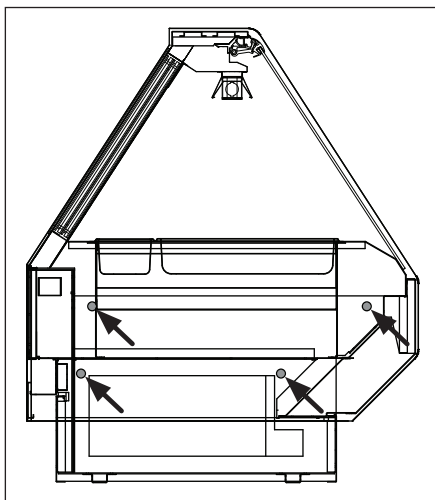
Fig. 3 Bolt locations
