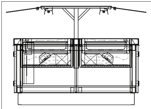
Fig. 12 Airflow pattern
