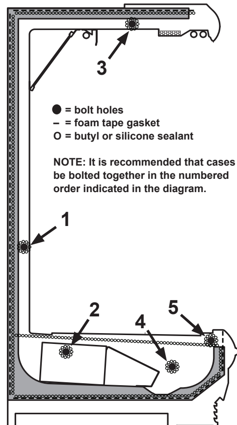
Fig. 2 Bolt holes, foam tape gasket and sealant
