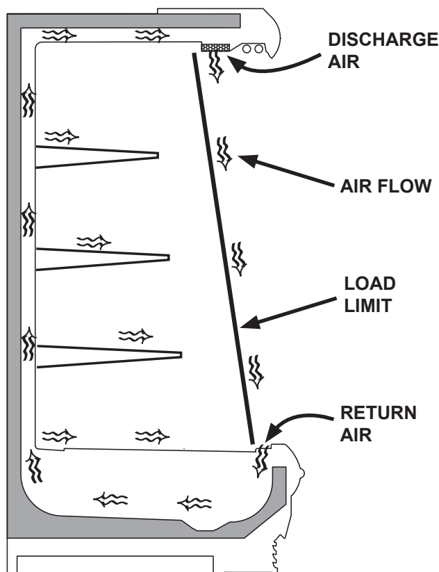
Fig. 19 Airflow
