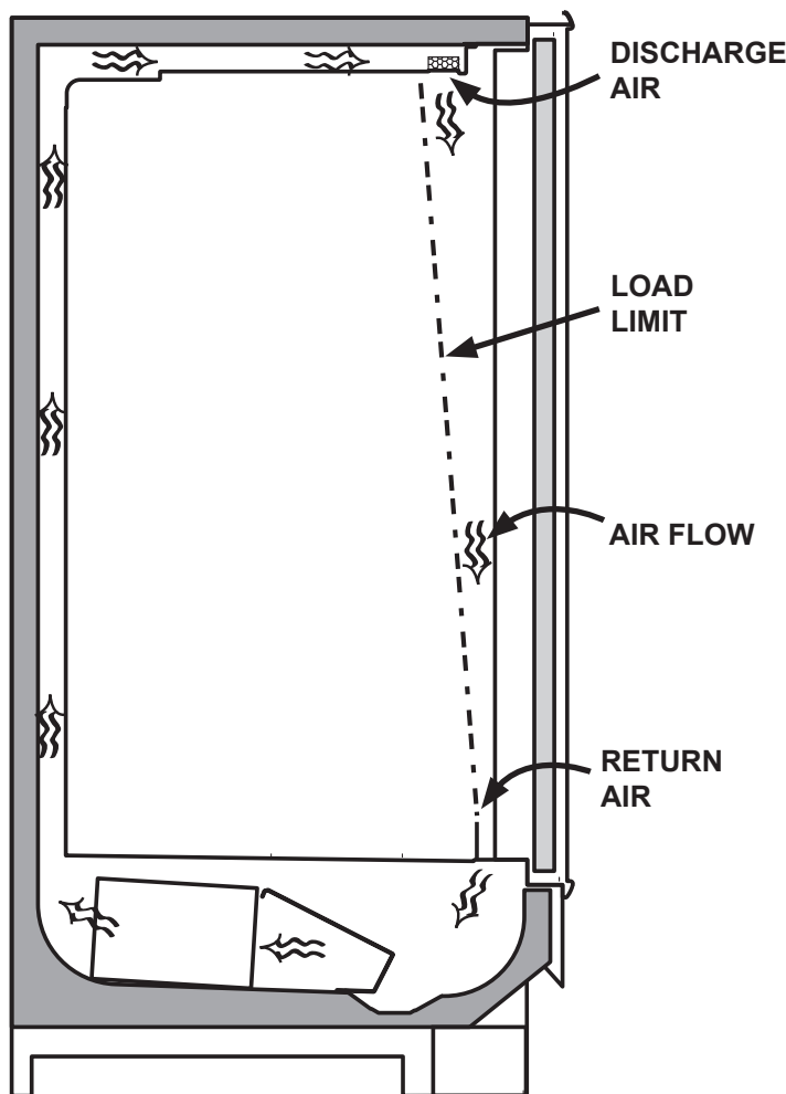
Fig. 15 Airflow
