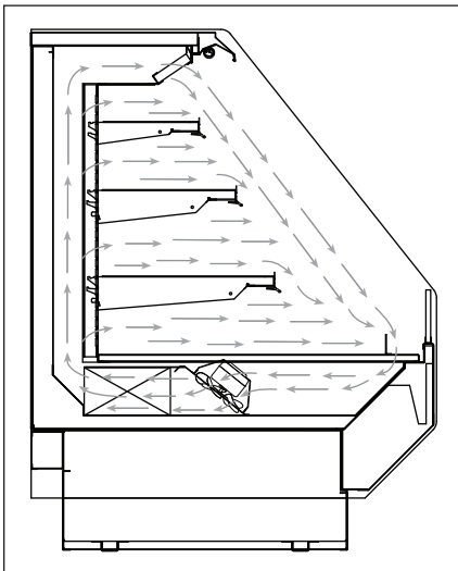
Fig. 12 Airflow pattern
