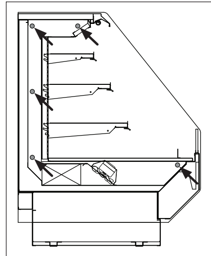
Fig. 3 Bolt locations
