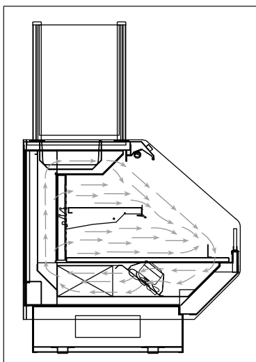
Fig. 12 Airflow pattern
