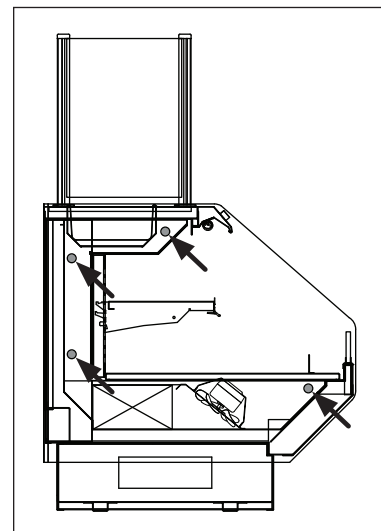
Fig. 3 Bolt locations
