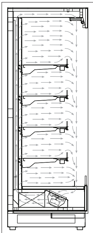
Fig. 12 Airflow pattern (QC-30-R)
