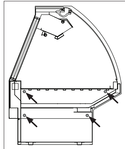
Fig. 3 Bolt locations
