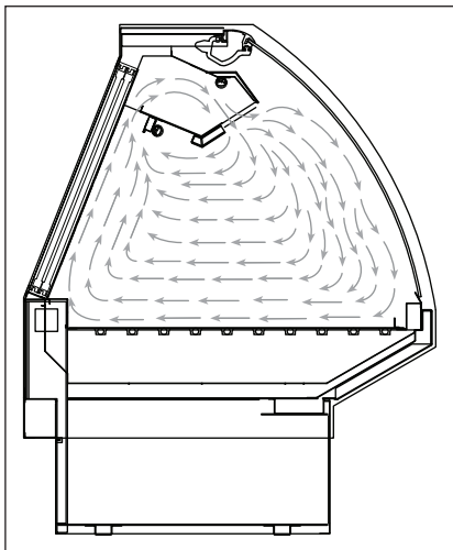
Fig. 11 Airflow Pattern
