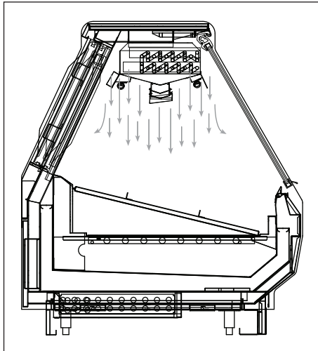
Fig. 12 Airflow pattern
