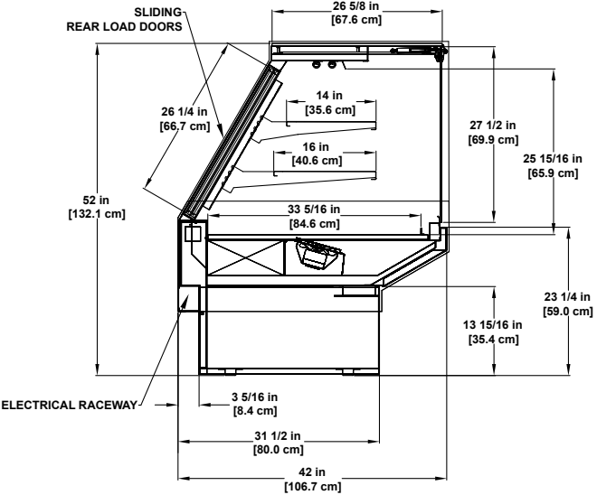
SMD-R Refrigerated/Vertical Glass Multi-deck Display
