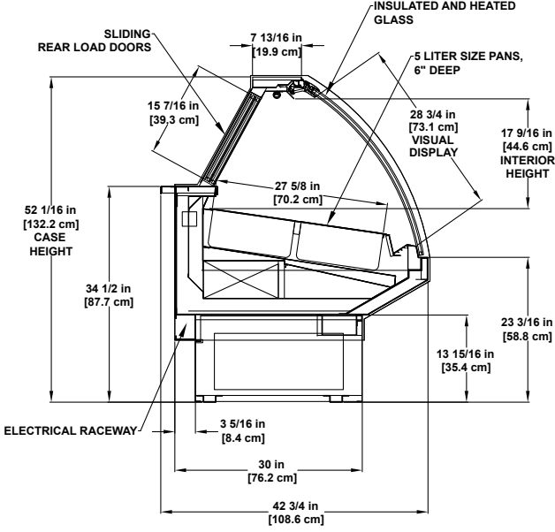
SSD-LT-R Gelato Frozen Single-deck Display
