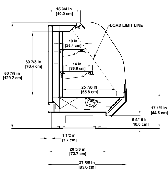
BLF-SR | Refrigerated Multi-deck Display
