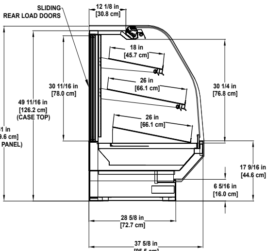
BLF-D Dry Multi-deck Display
