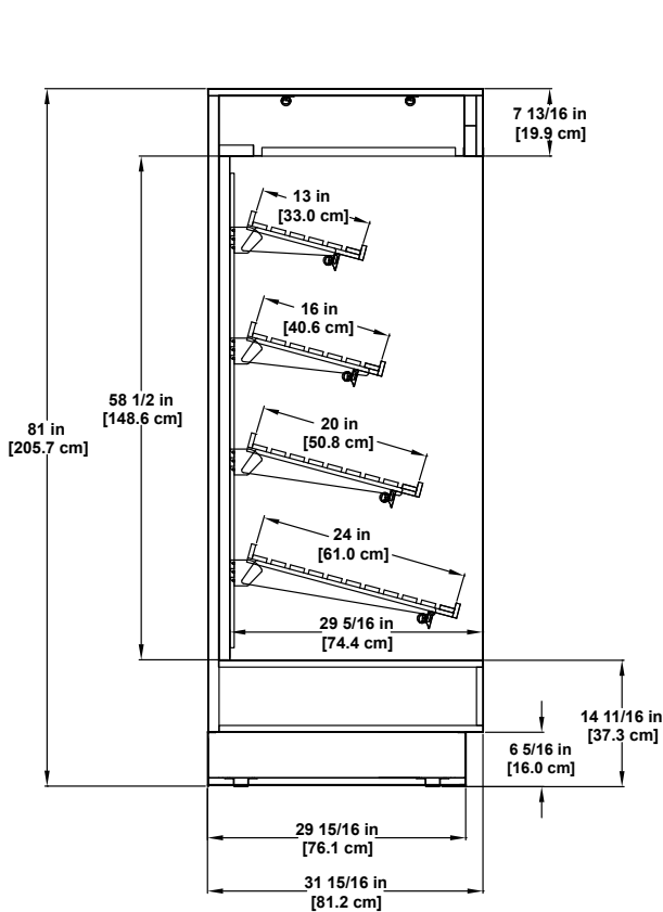
BWS-B Dry Multi-deck Display
