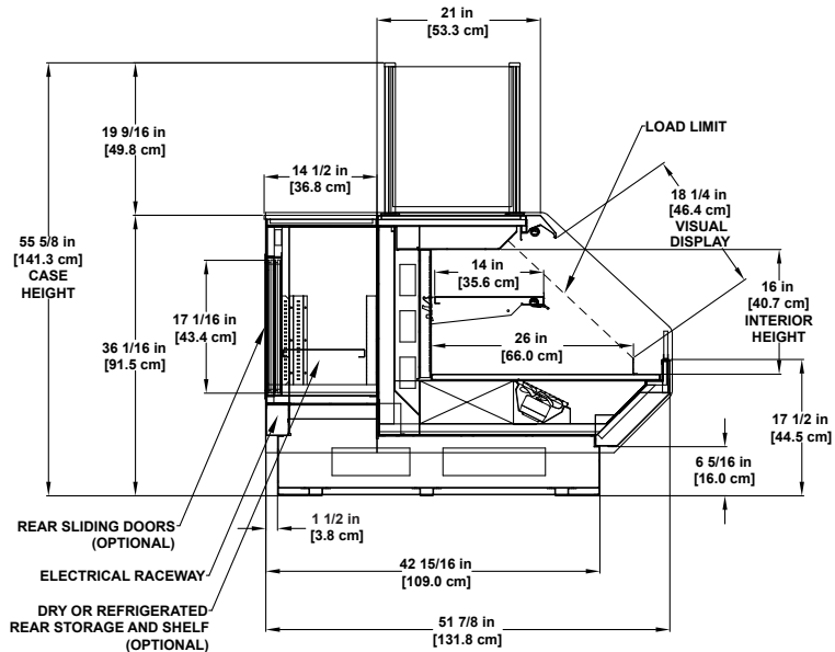
BLF-CR | Refrigerated Multi-deck Display
