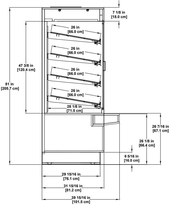
BWU-D Dry Multi-deck Display
