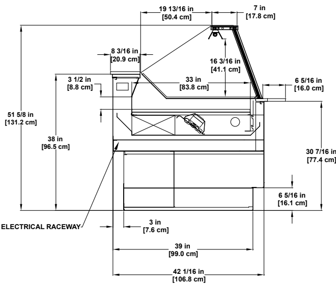
PC-G-R Refrigerated Single-deck Display
