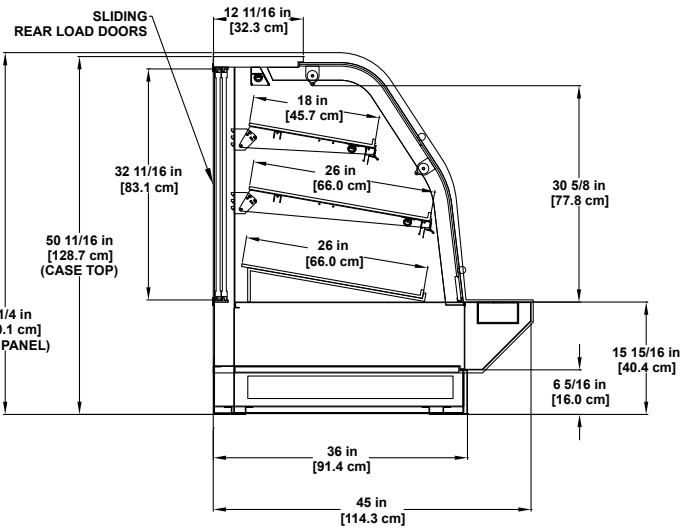
BLF-RB | Dry Multi-Deck Display
