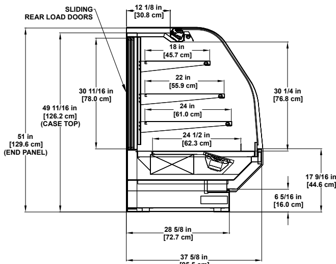
BLF-R Refrigerated Multi-deck Display
