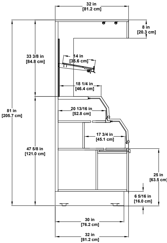
BWS-RB Dry Multi-deck Display
