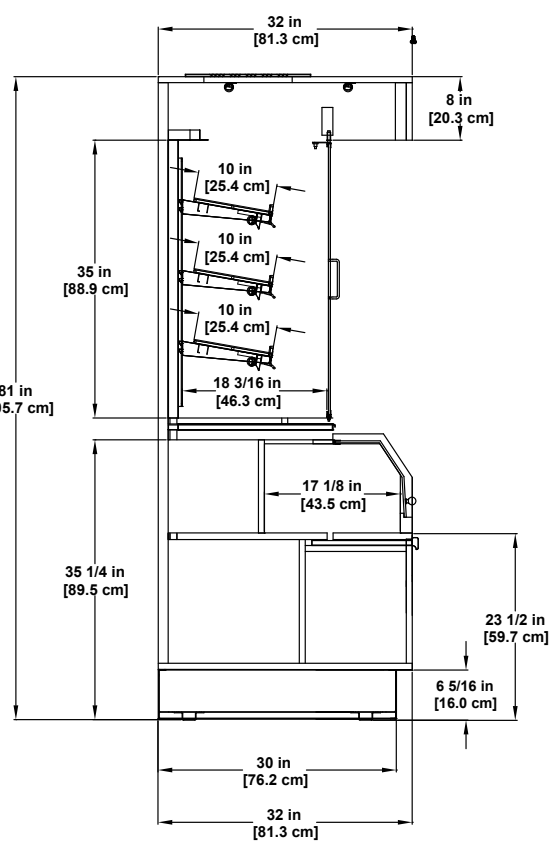
BWU-RB Dry Multi-deck Display
