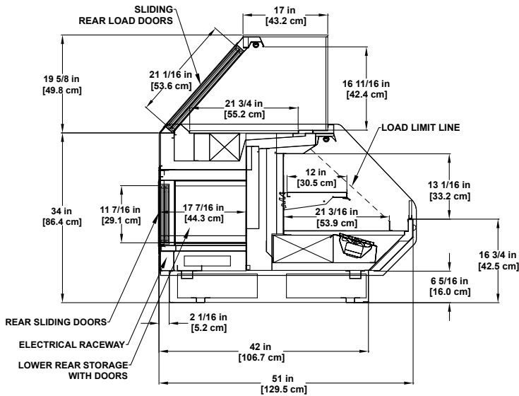
PTD-GSD-R | Refrigerated Service Dome and Self-service Base
