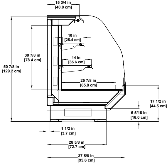
BLF-SD | Dry Multi-deck Display
