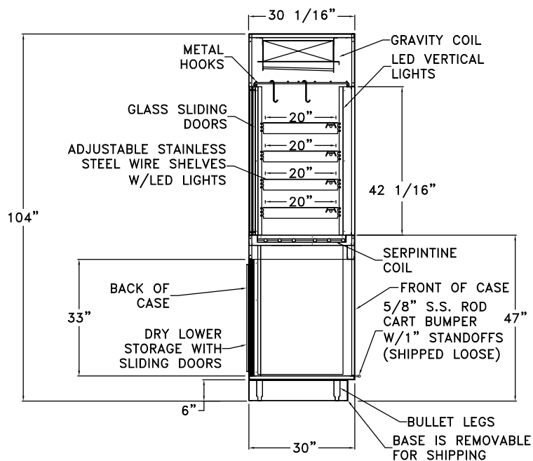
AGB-RG Refrigerated Multi-deck Display Drawing #124153
