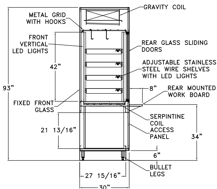
AGB-RG Refrigerated Multi-deck Display Drawing #130994
