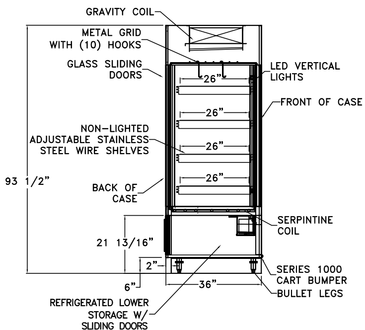
AGB-RG Refrigerated Multi-deck Display Drawing #136757
