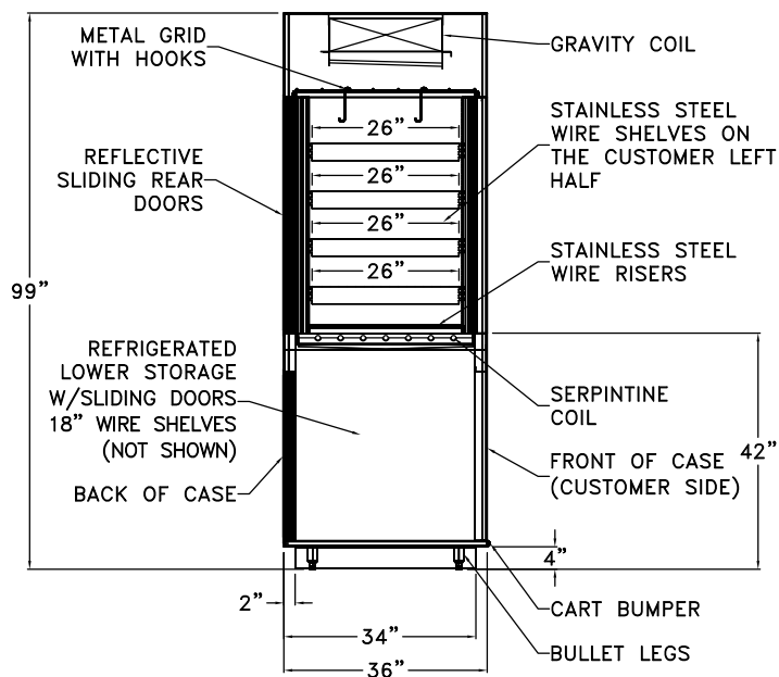
AGB-RG Refrigerated Multi-deck Display Drawing #131620
