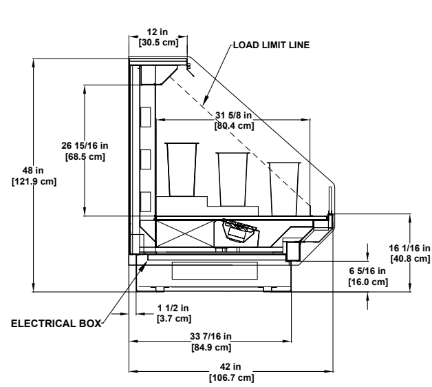
FT-R Refrigerated Multi-deck Display
