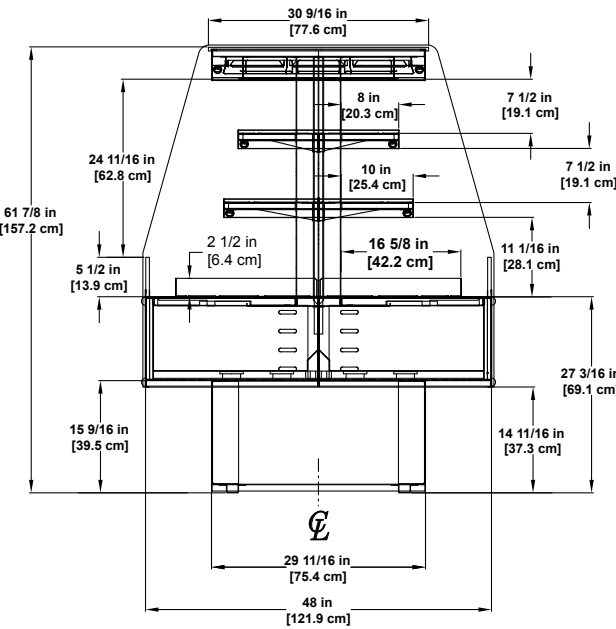
HVI-3-406R-RAD HVI-3-408R-RAD Refrigerated Multi-deck Display with Two End Caps
