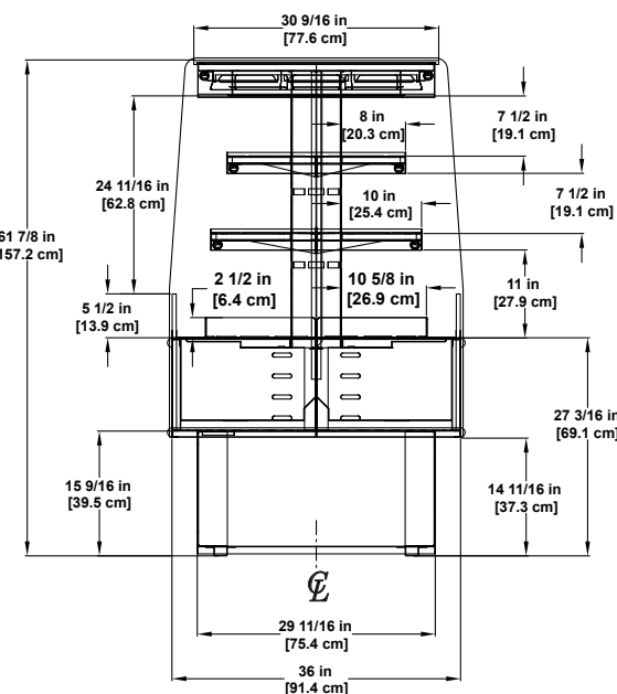
HVI-3-304SC-EC HVI-3-305SC-EC Refrigerated Multi-deck Display with One End Cap
