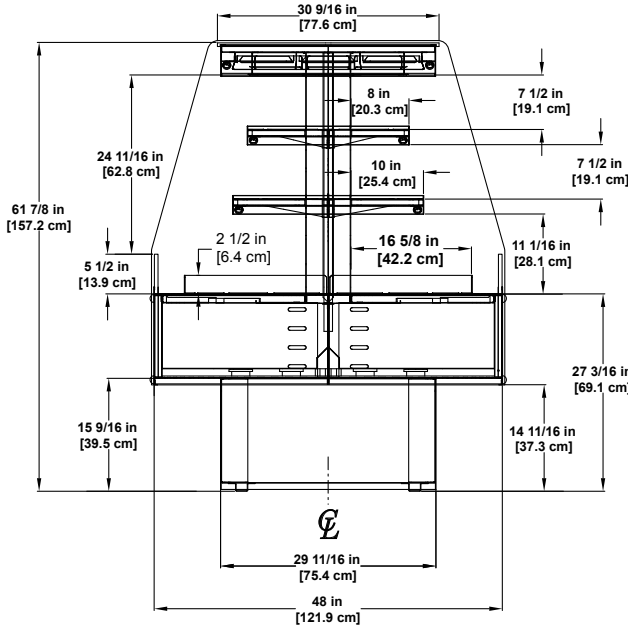
HVI-3-406SC-EC Refrigerated Multi-deck Display with One End Cap
