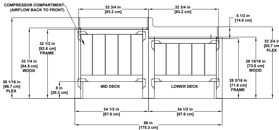
OB-R-2, 4 & 6 OB-SC-2 & 4 Refrigerated Single-deck Display
