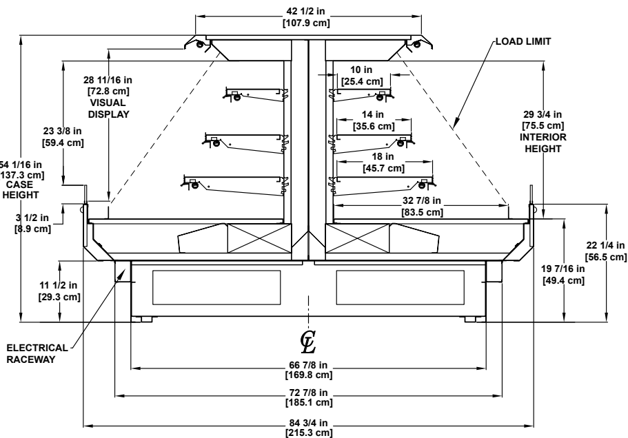
PFI-R-7 Refrigerated Multi-deck Display
