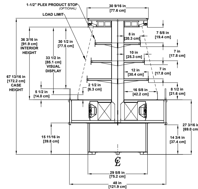
HVI-3-406R/S-RAD HVI-3-408R-RAD Refrigerated Multi-deck Display with Two End Caps
