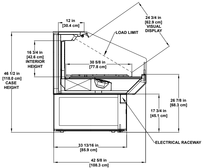
HSC Refrigerated Single-deck Display. Available in Remote and Self-contained.
