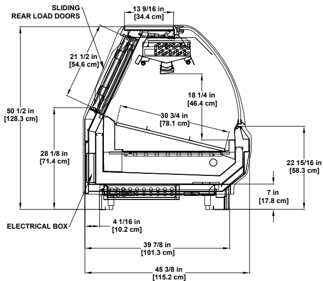
SSAM-RG Refrigerated Coolgenix® Single-deck Combo Display.
