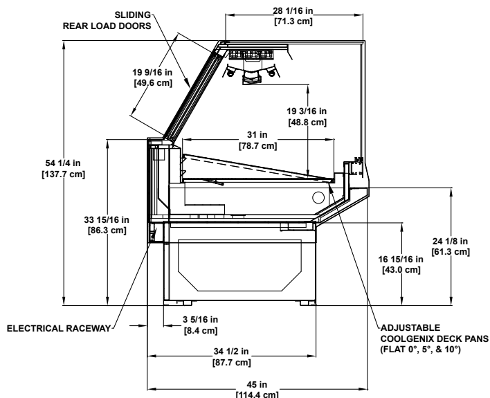
GMD-RGC Refrigerated Coolgenix® Multi-deck Display.
