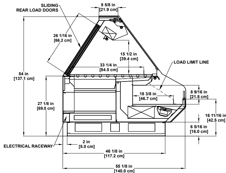
SD-RG Refrigerated Gravity Coil Multi-deck Combo Display.
