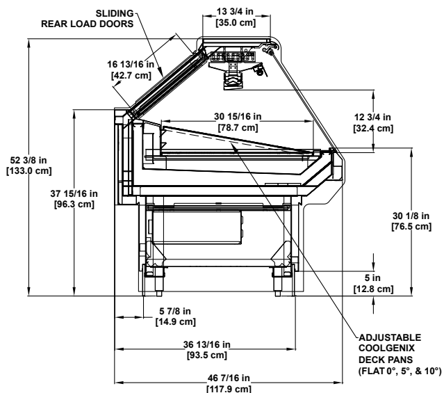
SSGC | Refrigerated Coolgenix® Single-deck Display.
