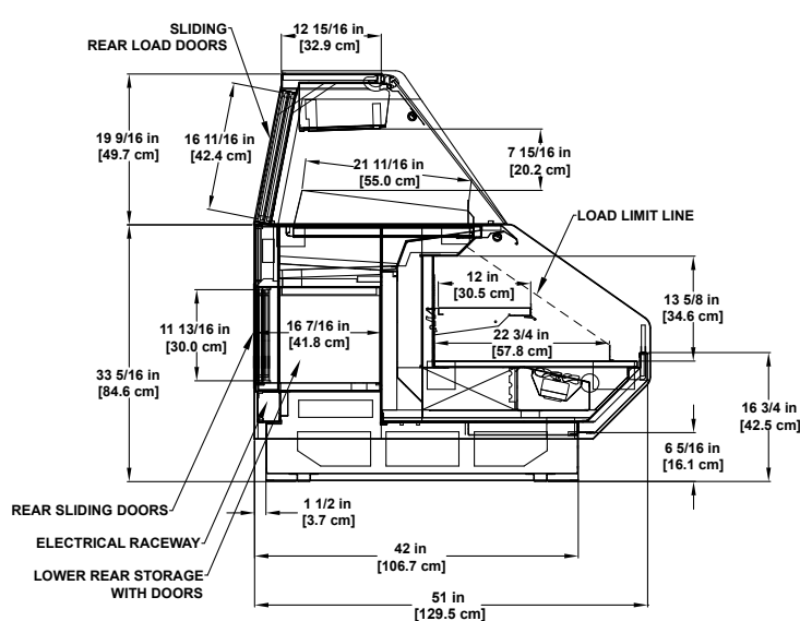
PTD-RG Refrigerated Gravity Coil Multi-deck Combo Display.
