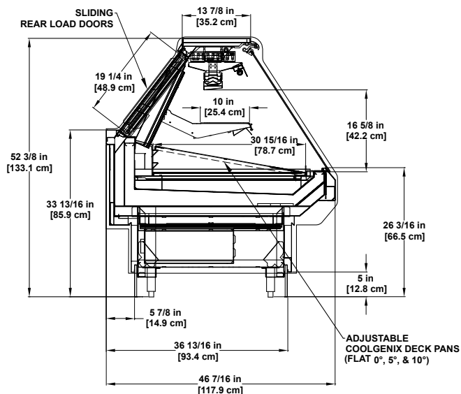
S2SGC Refrigerated Coolgenix® Single-deck Display.
