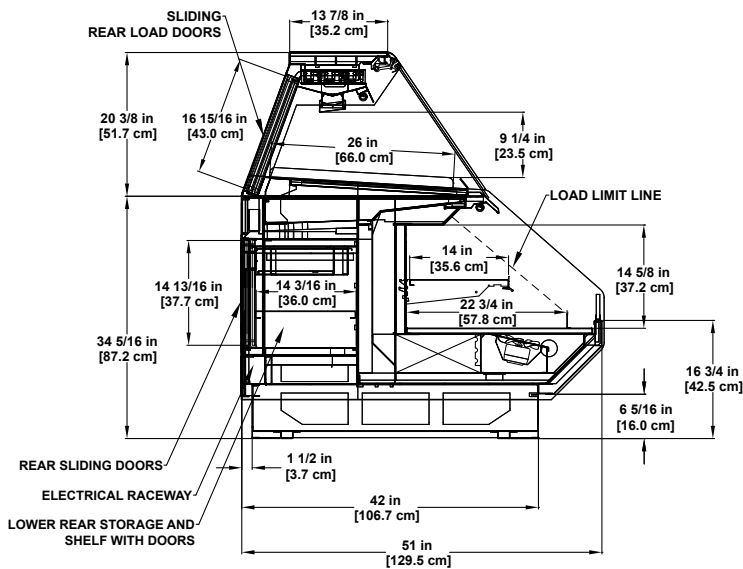
PTD-RGC Refrigerated Coolgenix® Multi-deck Combo Display.
