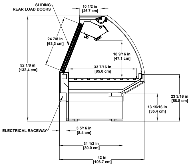
SMD-RG | Refrigerated Gravity Coil Single-deck Display. Also available in vertical glass option.
