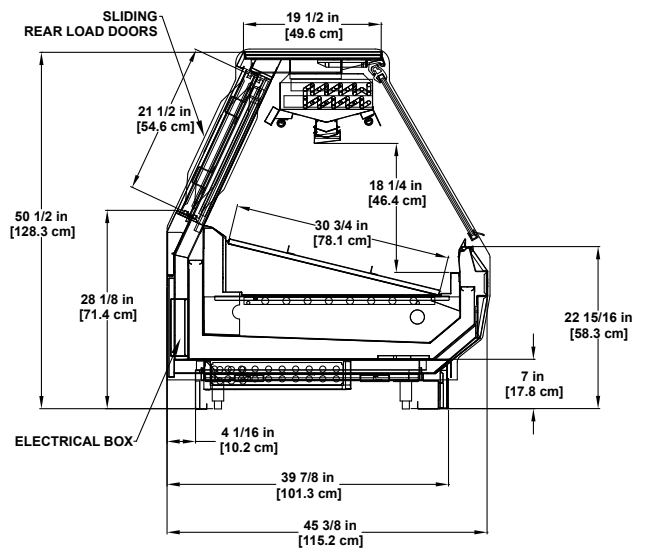
SSFM-RG Refrigerated Gravity Coil Single-deck Display.
