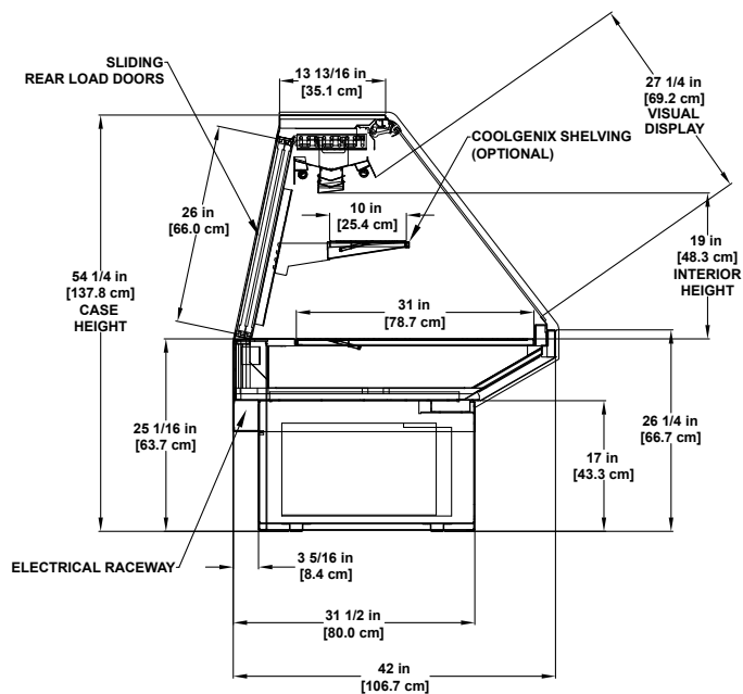
SMD-RGC | Refrigerated Gravity Coil Single-deck Display. Also available in vertical glass option.
