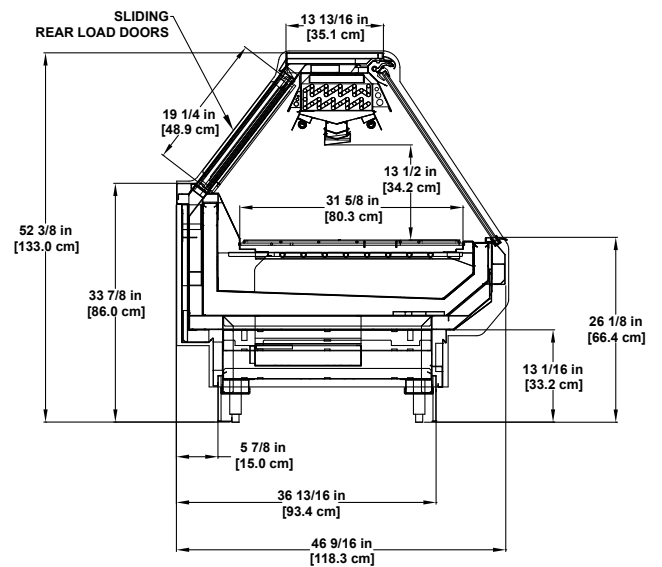
S2SG-R Refrigerated Gravity Coil Single-deck Display.
