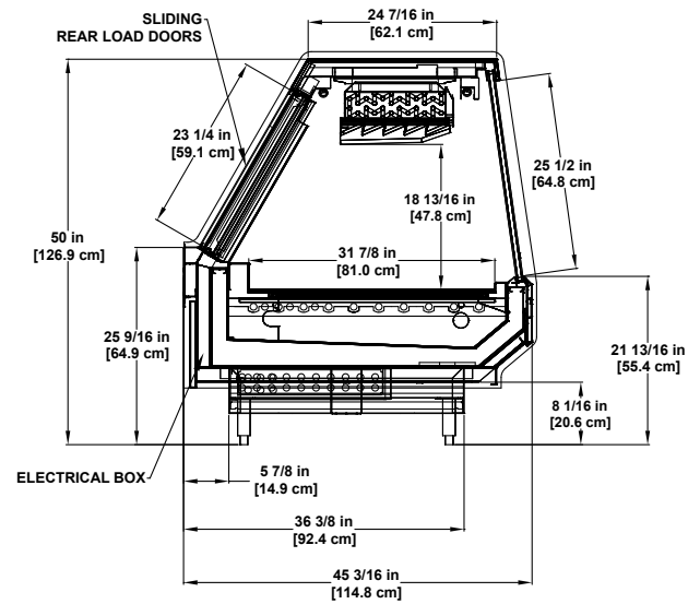
SGMO Refrigerated Gravity Coil Single-deck Display.
