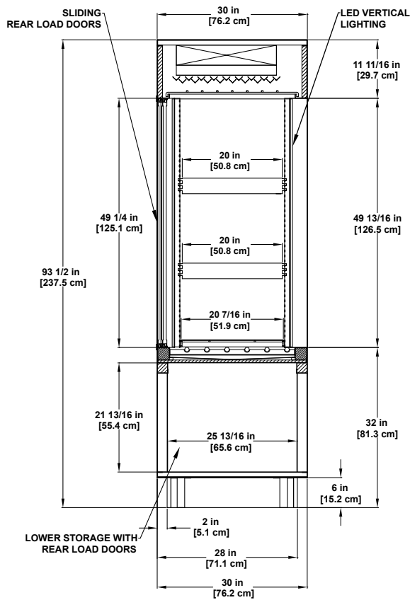
AGB-RG | Refrigerated Gravity Coil Multi-deck Aged Meat Display
