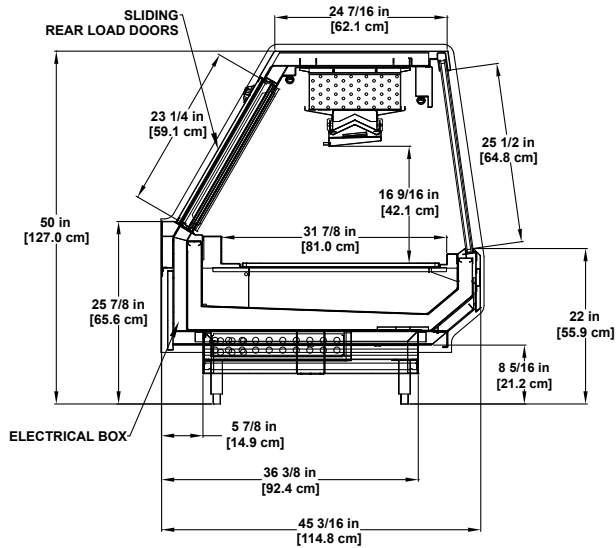
SGM Refrigerated Gravity Coil Single-deck Display. Available in 30° glass height.
