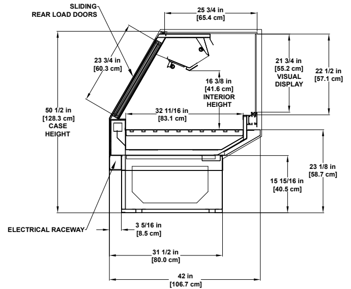
GMD-RG Refrigerated Gravity Coil Single-deck Display.
