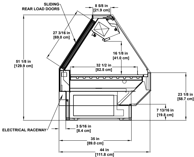
BMD-RG Refrigerated Gravity Coil Single-deck Display.
