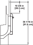
12" Glass Flat
