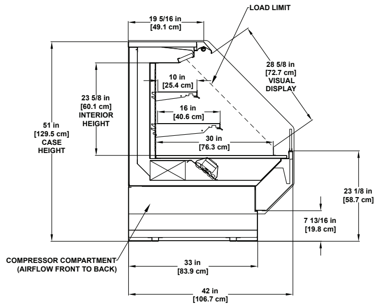
PF-R | Refrigerated Multi-deck Display 51" High
