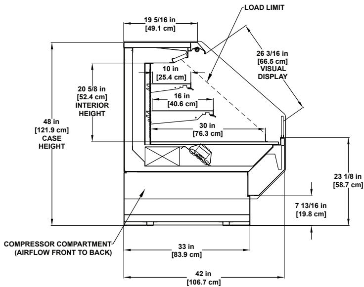
PF-R | Refrigerated Multi-deck Display 48" High
