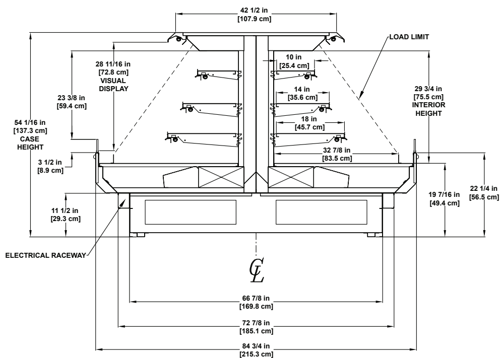
PFI-R-7 Refrigerated Multi-deck Display
