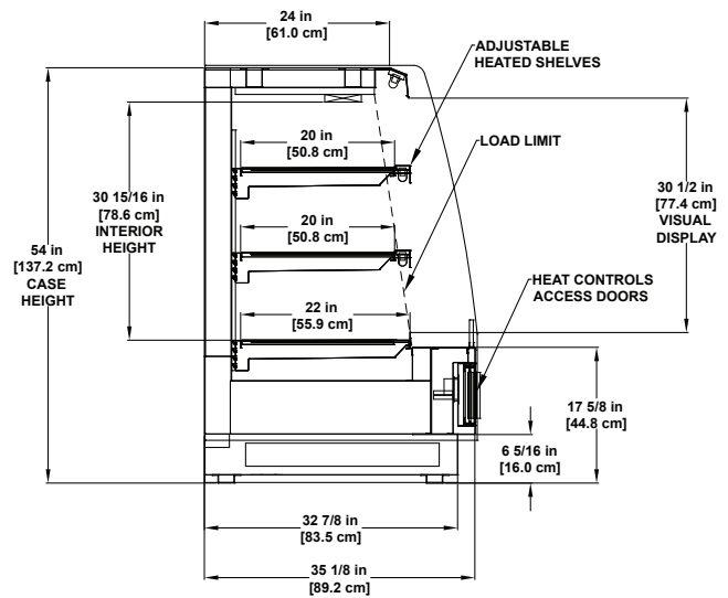
PFH-C | Hot Multi-deck Display Convection Heat
