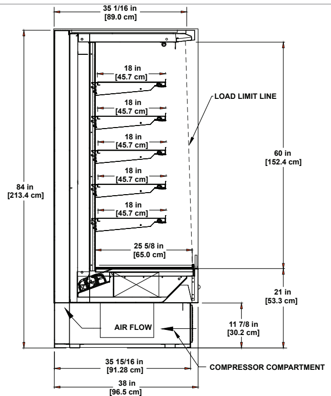
PF-SC-84 | Refrigerated Multi-deck Display
