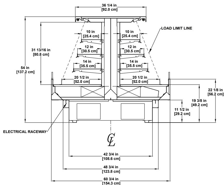
PFI-R-5 Refrigerated Multi-deck Display
