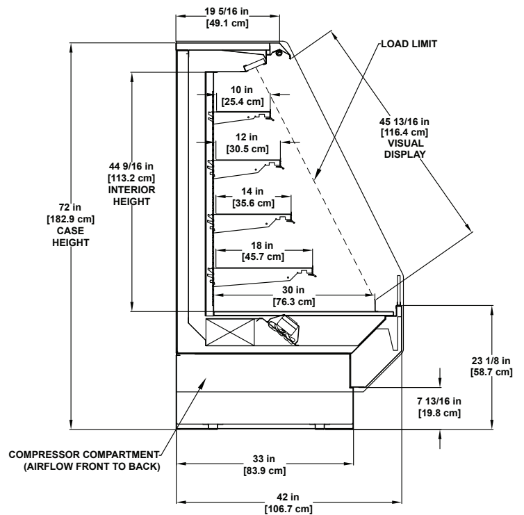
PF-R | Refrigerated Multi-deck Display 72" High
