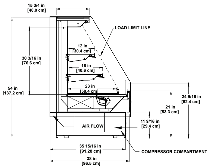
PF-SC-54 | Refrigerated Multi-deck Display
