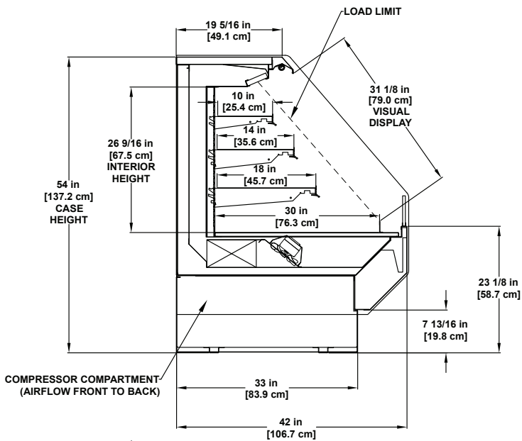
PF-R | Refrigerated Multi-deck Display 54" High
