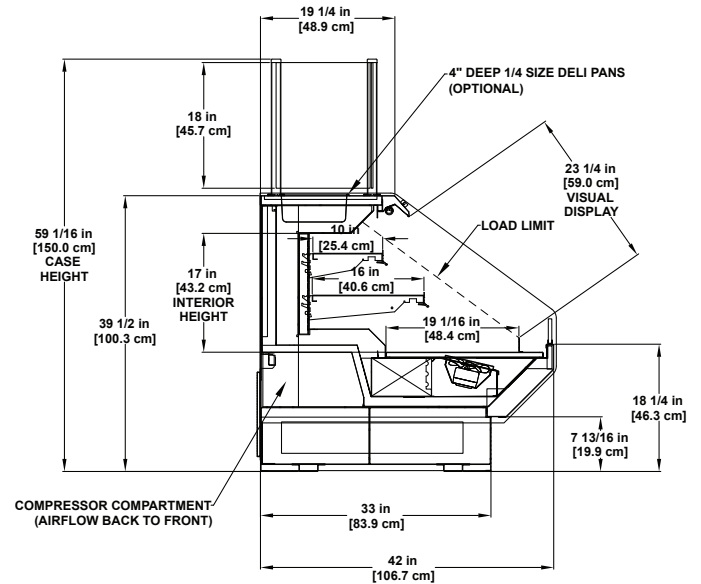
PT-SC | Refrigerated 4' & 6' Multi-deck Display
