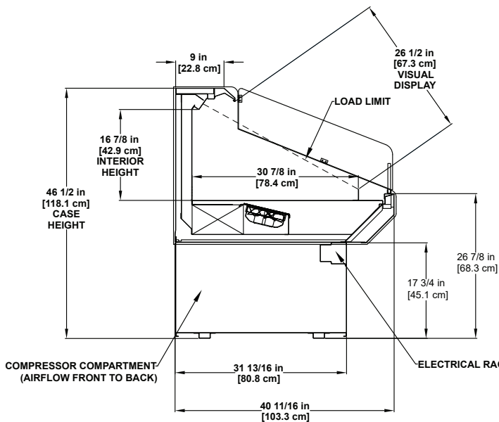
HS | 46-1/2"H x 40-11/16"D Refrigerated 3' & 4' Single-deck Display
