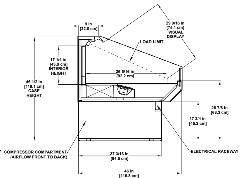
HS | 46-1/2"H x 46"D Refrigerated 2', 3', 4' & 6' Single-deck Display
