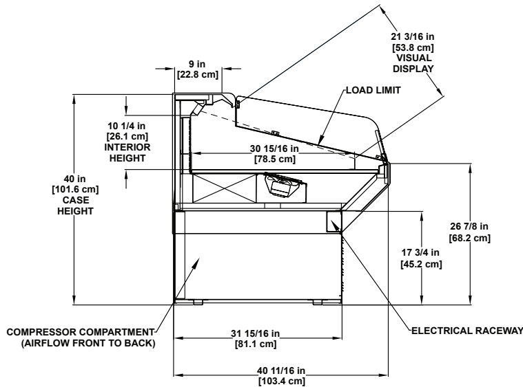
HS | 40"H x 40-11/16"D Refrigerated 2', 3', 4' & 6' Single-deck Display
