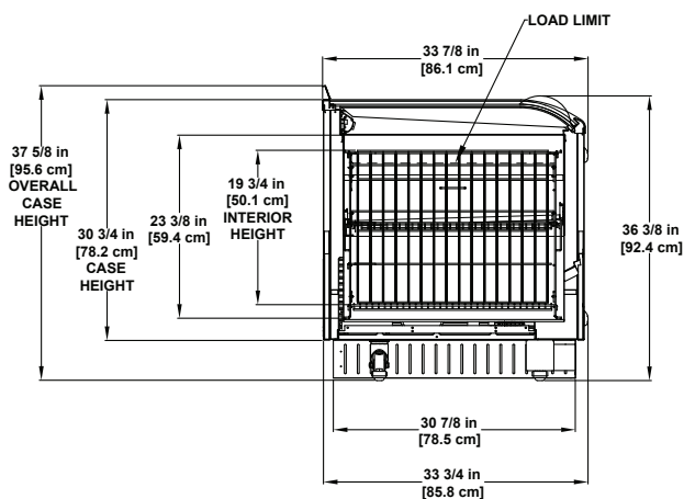
CNZLA | Dual-Temp 4', 7', & 8' Single-deck Display In-line or Island Display
