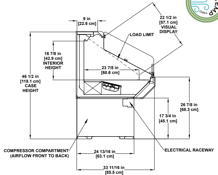
HS | 46-1/2"H x 33-11/16"D Refrigerated 3' & 4' Single-deck Display
