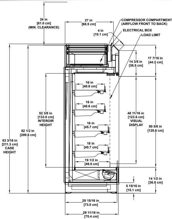
QTM-30 | Refrigerated 47" Multi-deck Display
