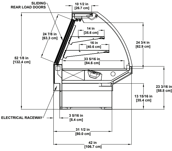
SMD-R Refrigerated / Curved Glass Multi-deck Display Application: Deli
