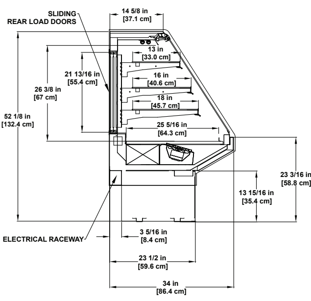
SMD-R-Candy Refrigerated / Flat Glass Multi-deck Display Application: Candy
