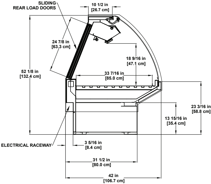
SMD-RG Refrigerated / Curved Glass Single-deck Display Application: Deli, Meat, and Seafood
