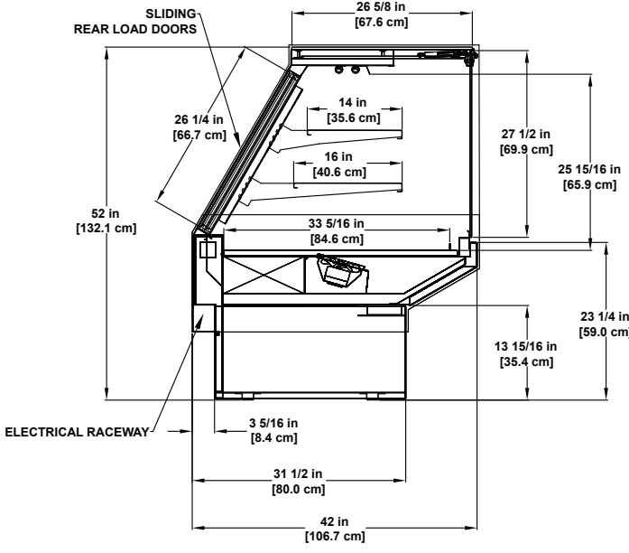
SMD-R Refrigerated / Vertical Glass Multi-deck Display Application: Deli and Bakery
