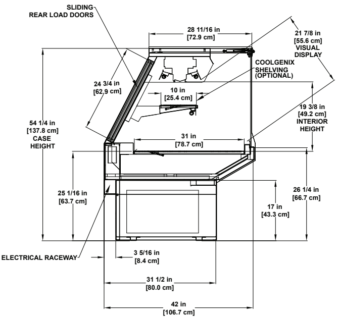
SMD-RGC Refrigerated Coolgenix / Vertical Glass Multi-deck Display Application: Meat and Seafood
