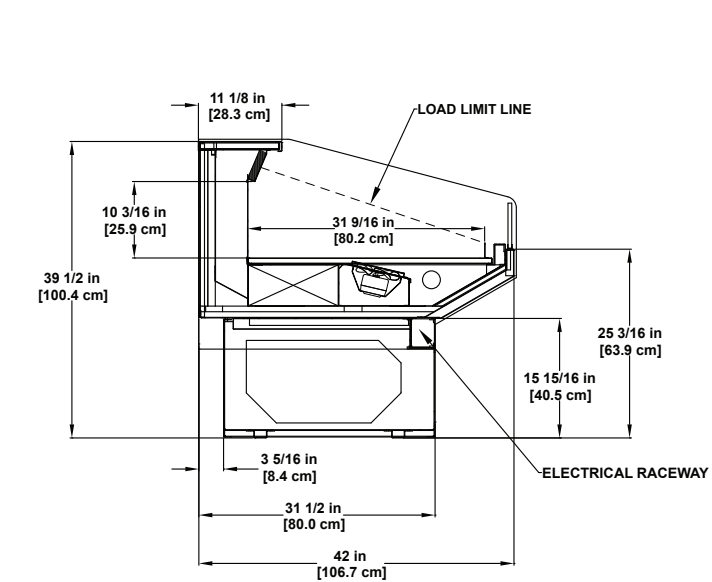
DLPC-R | Refrigerated Single-deck Display Application: Bakery, Beverage, Deli, Meat, and Seafood
