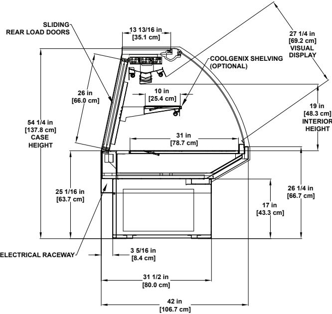
SMD-RGC Refrigerated Coolgenix / Curved Glass Multi-deck Display Application: Meat and Seafood
