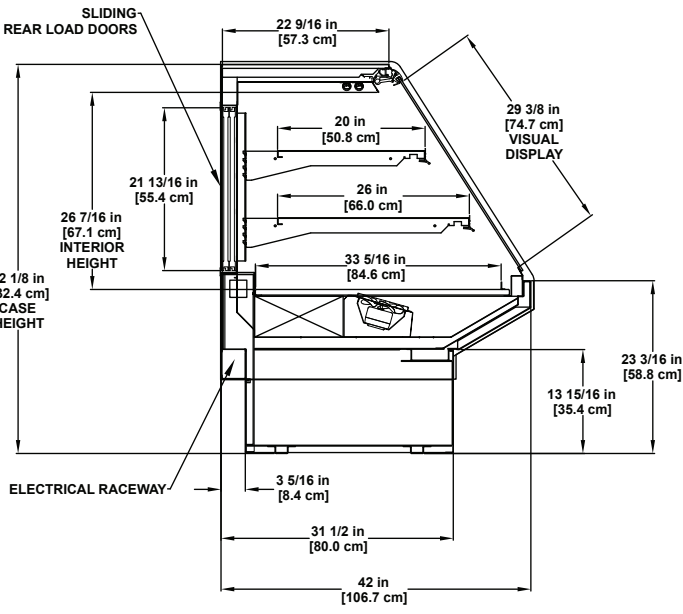
SMD-R-Bakery Refrigerated / Flat Glass Multi-deck Display Application: Bakery
