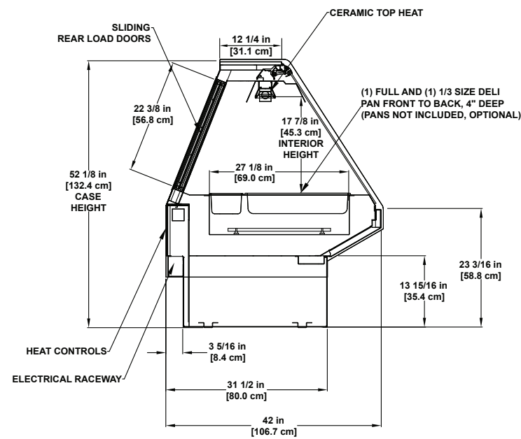
SMDH | Hot / Flat Glass Single-deck Display Application: Deli Hot Foods
