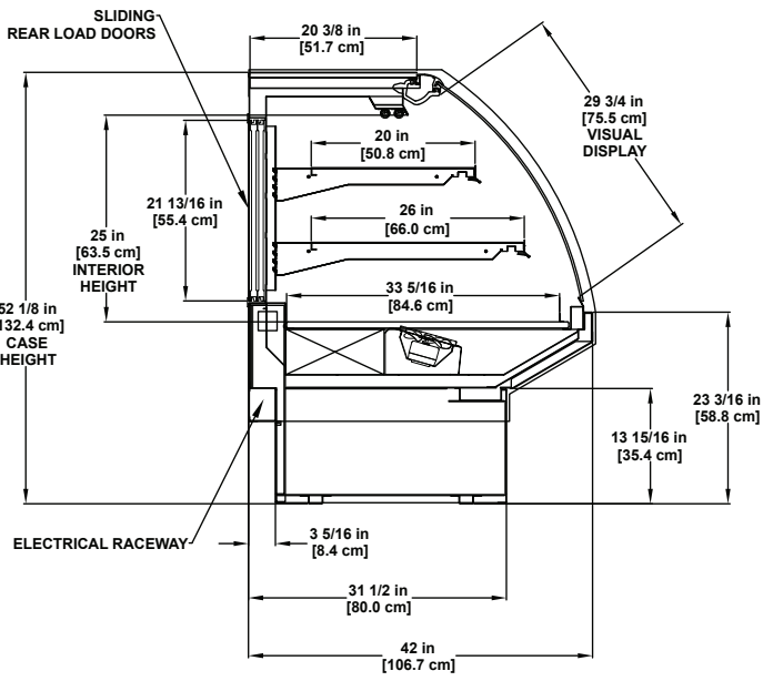
SMD-R-Bakery Refrigerated / Curved Glass Multi-deck Display Application: Bakery
