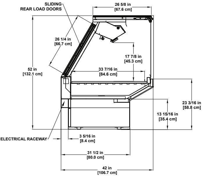
SMD-RG Refrigerated / Vertical Glass Single-deck Display Application: Deli, Meat, and Seafood
