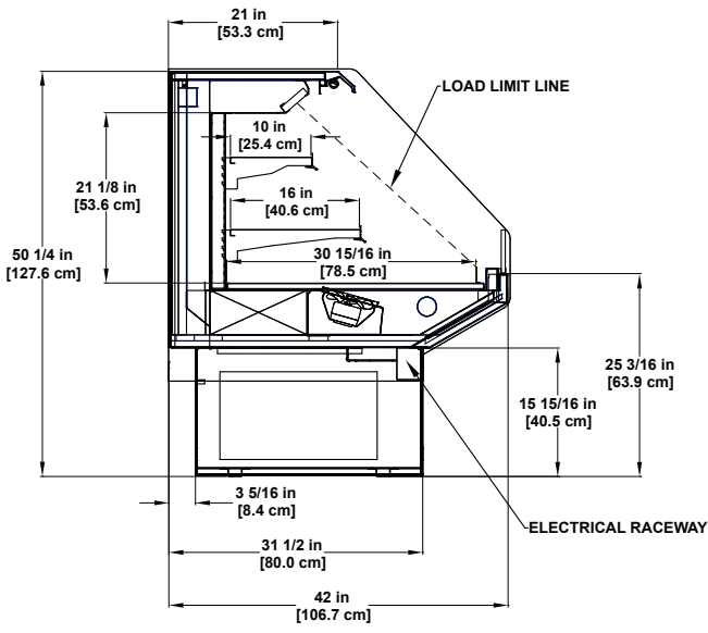
DLPF-R | Refrigerated Multi-deck Display Application: Bakery, Beverage, and Deli
