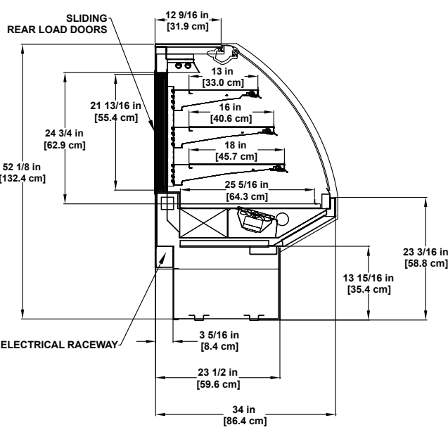
SMD-R-Candy Refrigerated / Curved Glass Multi-deck Display Application: Candy
