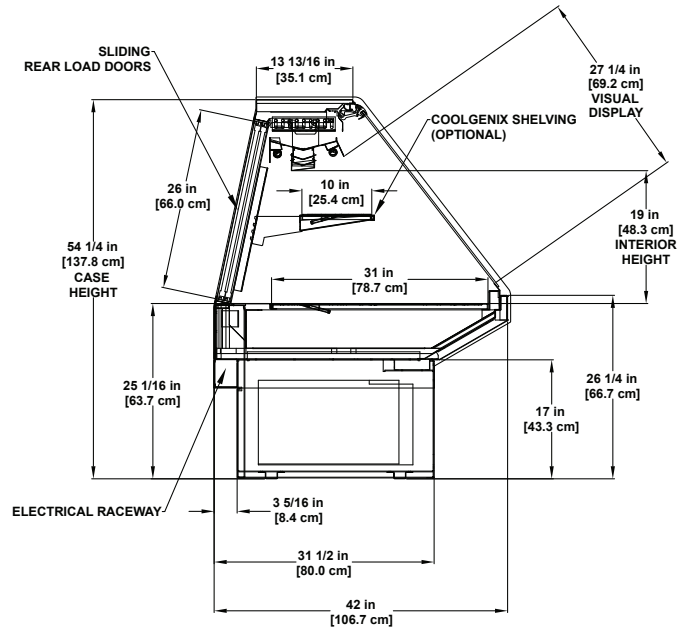
SMD-RGC Refrigerated Coolgenix / Flat Glass Multi-deck Display Application: Meat and Seafood
