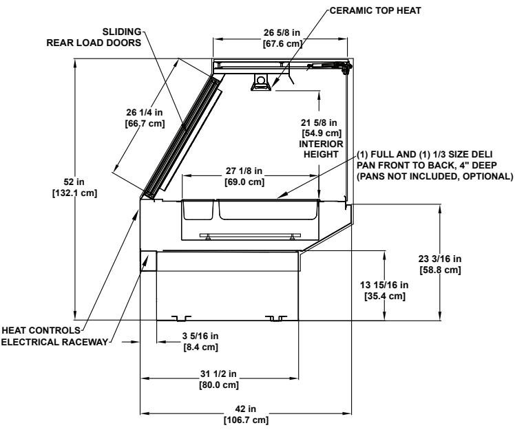
SMDH | Hot / Vertical Glass Single-deck Display Application: Deli Hot Foods
