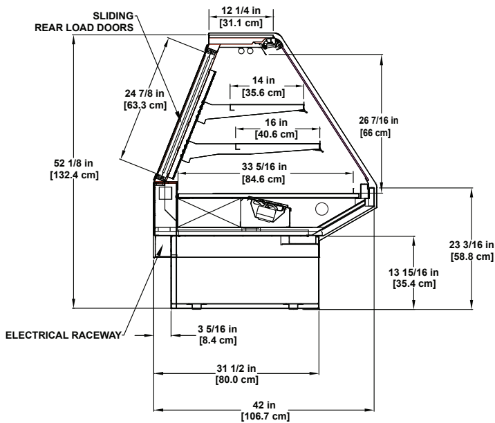
SMD-R Refrigerated / Flat Glass Multi-deck Display Application: Deli
