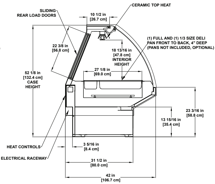
SMDH | Hot / Curved Glass Single-deck Display Application: Deli Hot Foods
