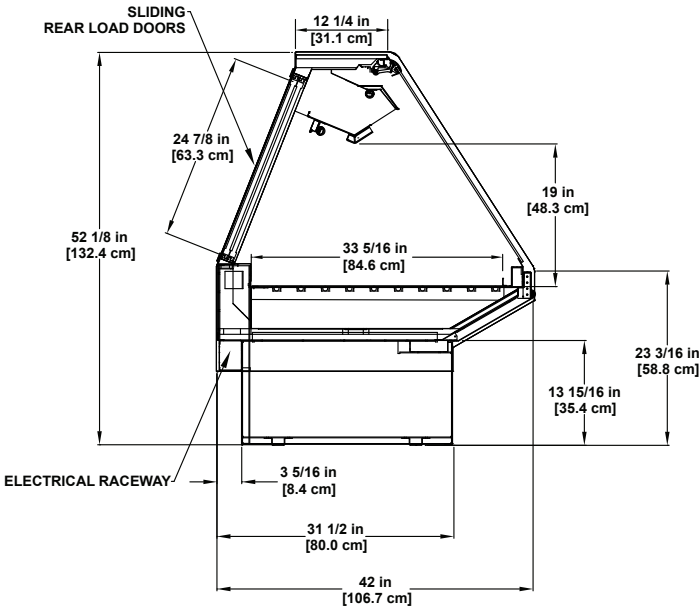
SMD-RG Refrigerated / Flat Glass Single-deck Display Application: Deli, Meat, and Seafood
