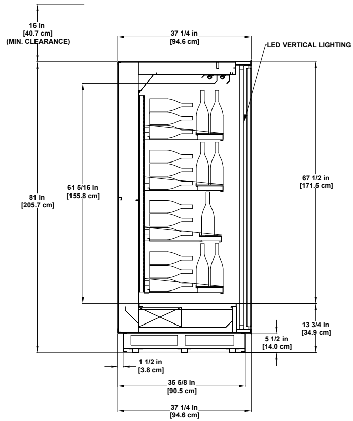
NFD-R Refrigerated Multi-deck Display
