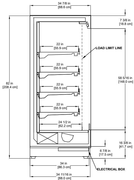
QC-R Refrigerated Multi-deck Display
