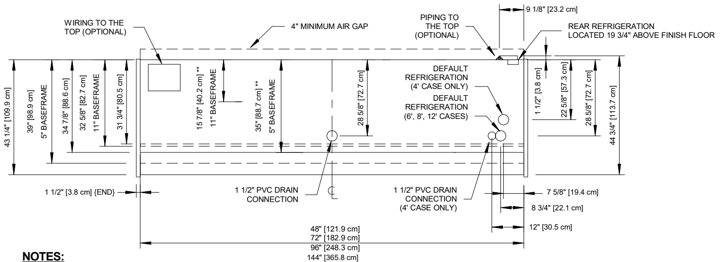
11" BASEFRAME
