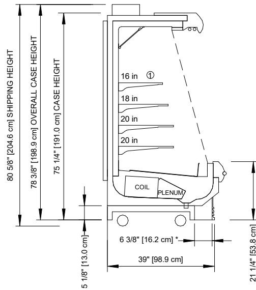
5" BASEFRAME
